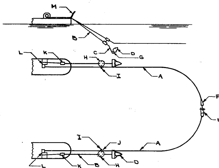
Figure 7(B) TWIN SHIP LARGE SWEEPING GEAR, MODEL 5
