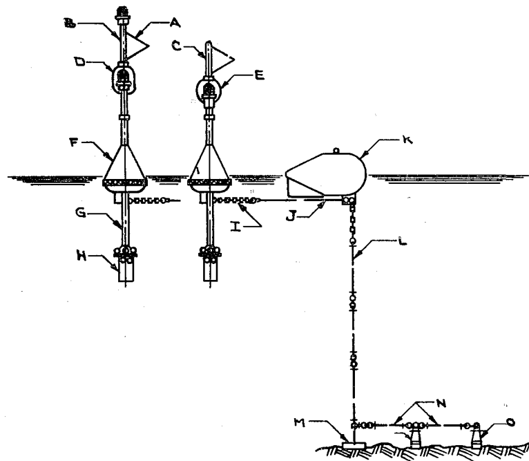
Figure 22(B) SWEEPING MARKER LIGHTS
