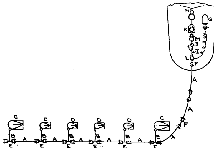
Figure 6(B) TWIN SHIP LARGE SWEEPING GEAR, MODEL 4
