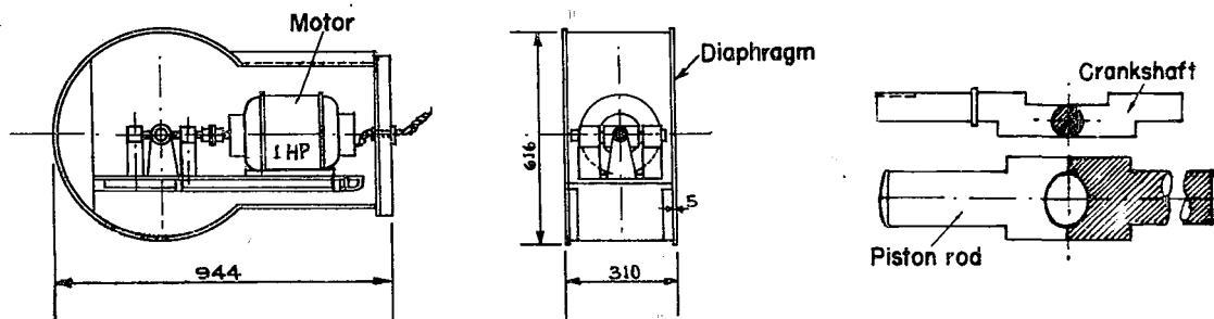
Figure 6(A) ACOUSTIC MINE SWEEPING DEVICES
