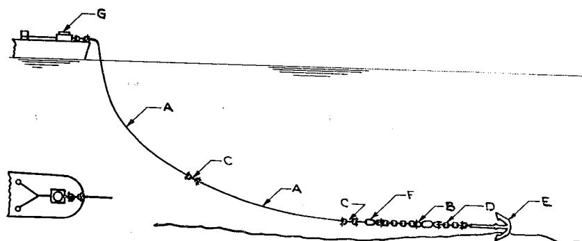
Figure 16(i) DEEP SEA SEARCH GEAR, MODEL 1
