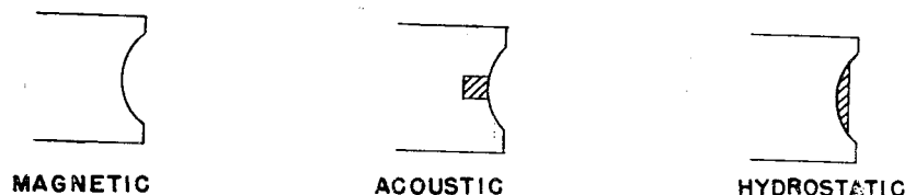
Figure 11 DIAGRAMS OF FIRING MECHANISM IN U.S. MINES
