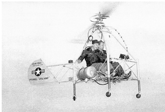
XH-20 Little Henry ramjet helicopter
