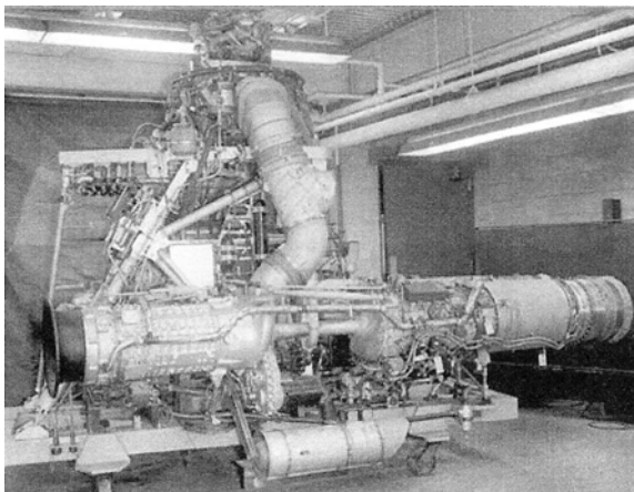
XHCH-1 power assembly.
